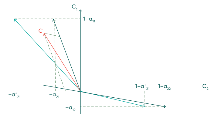
Fig. 3. Solution with positive outputs changing the second row of matrix A.
